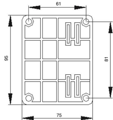
MOUNT BRACKET
